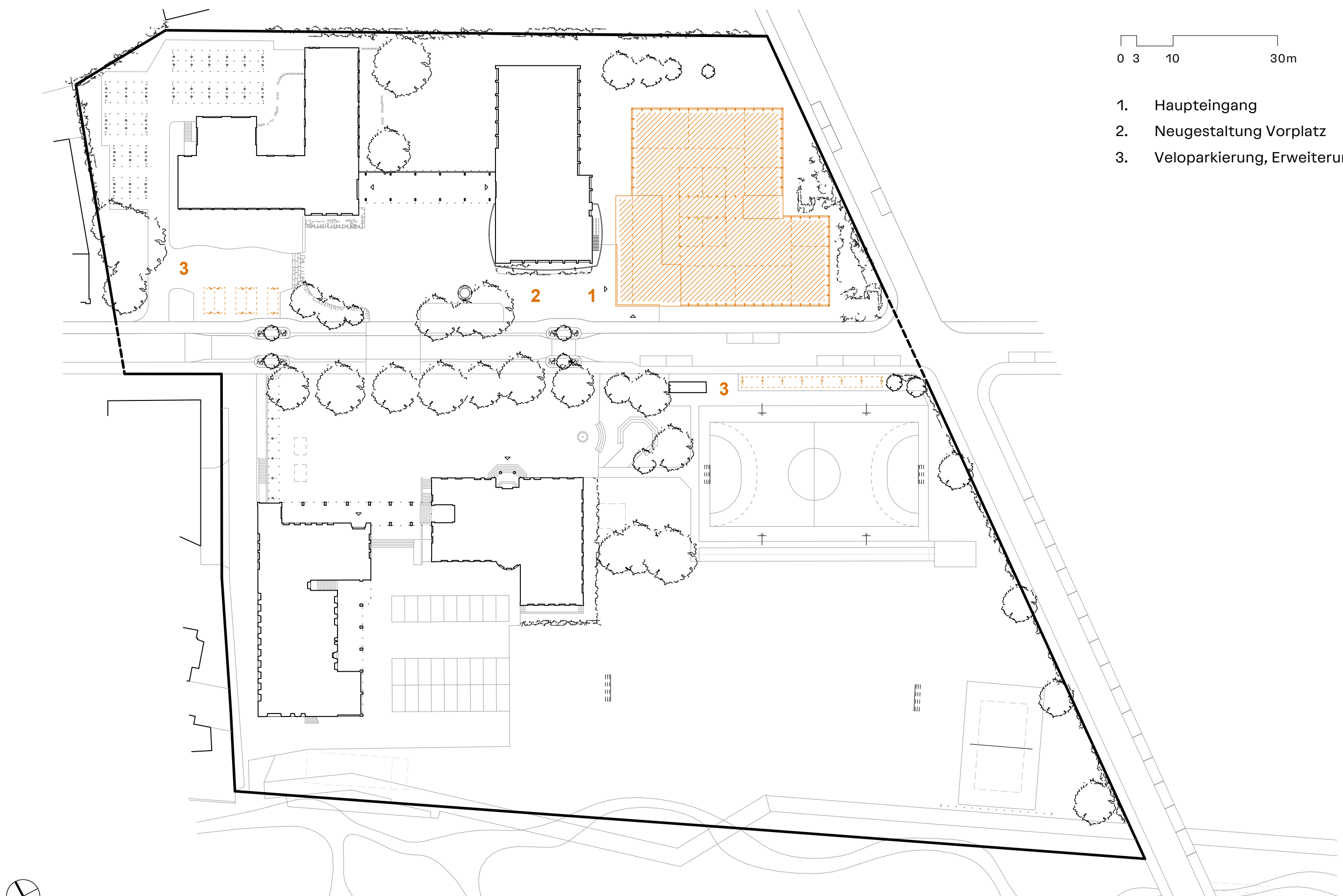
SITUATIONSPLAN
